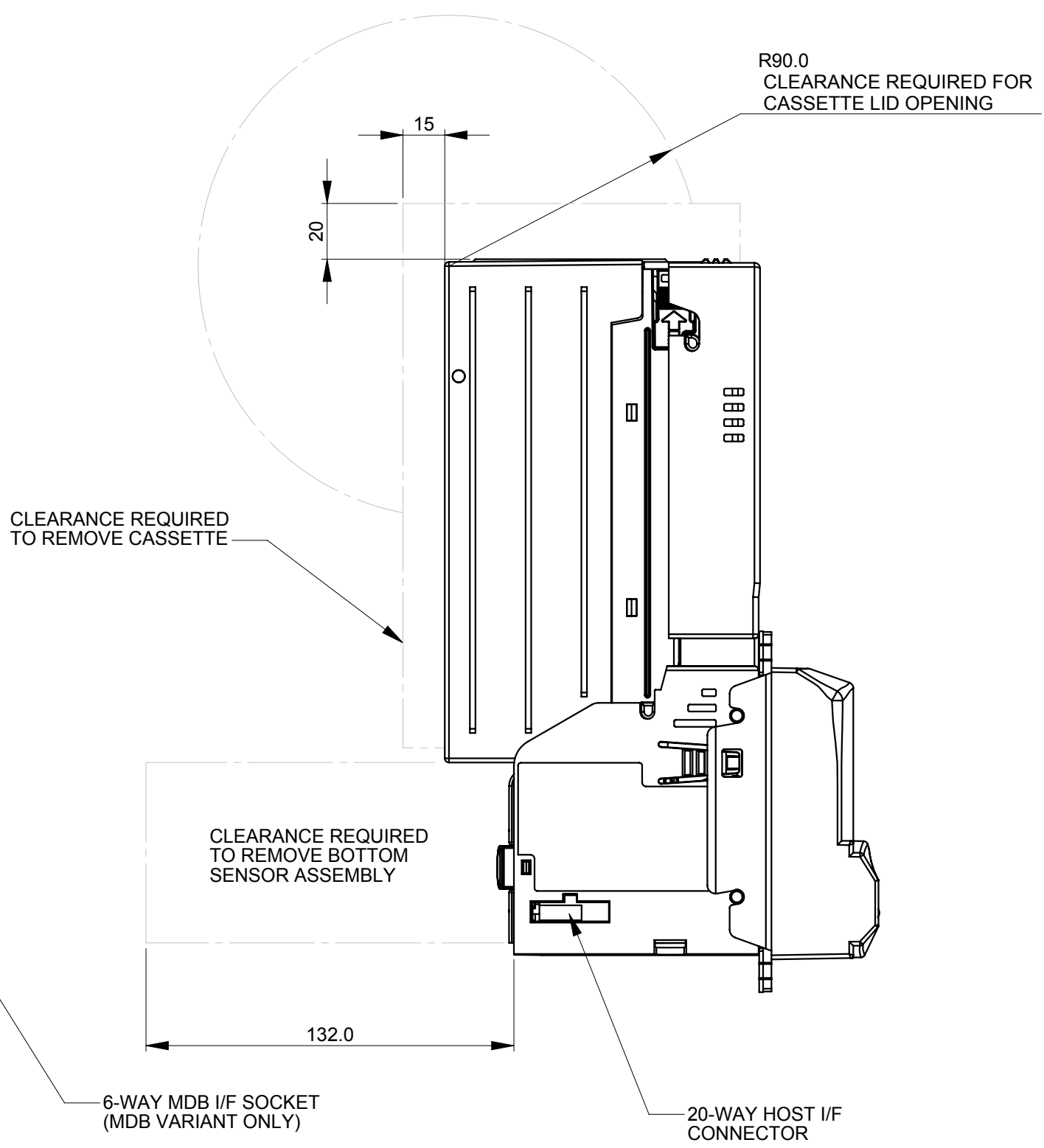
HOST MACHINE MOUNTING DETAILS
